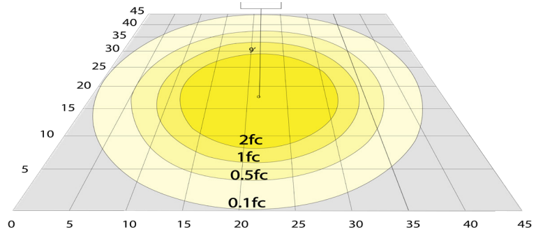
40W 5000K, Area 45'x 45' Mounting Height: 9'
